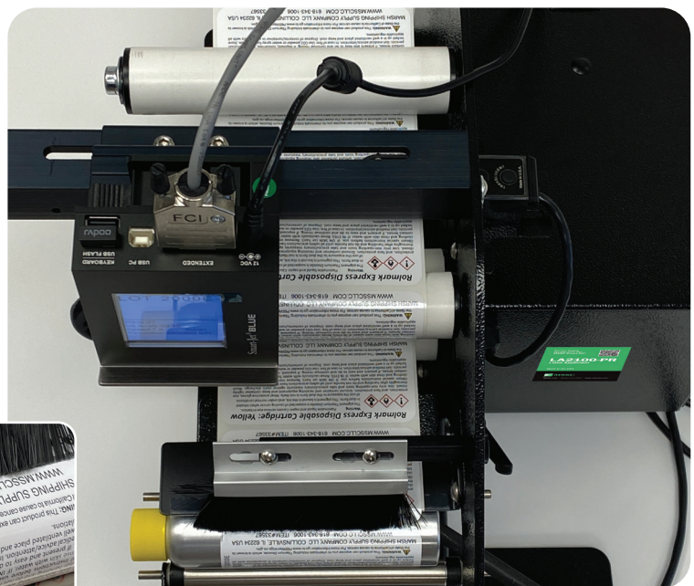
LA2100-PR Label Applicator
